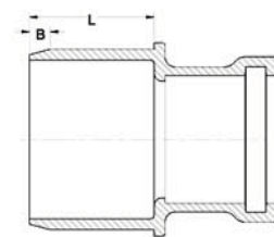
Reducer
