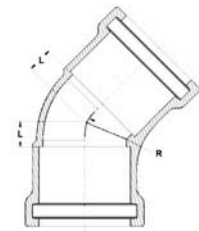
45 Bend
